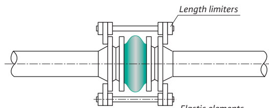
Expansion joint with length limitation without elastic elements (lateral expansion joint)
