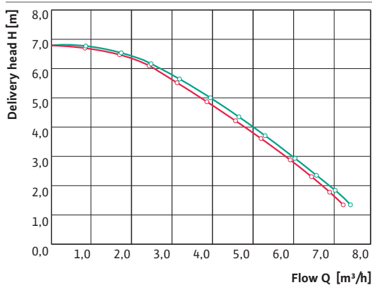
Sample curve for potential changes in a circulating pump
