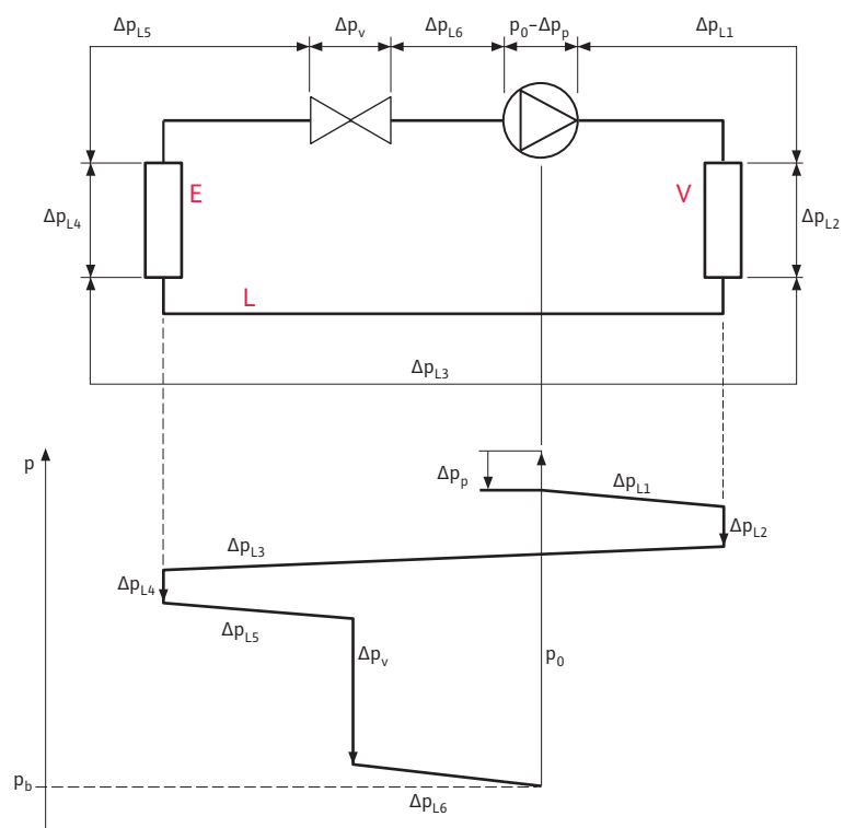
Pressure diagram
