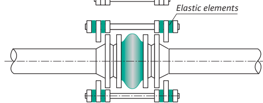
Expansion joint with length limitation with elastic elements
