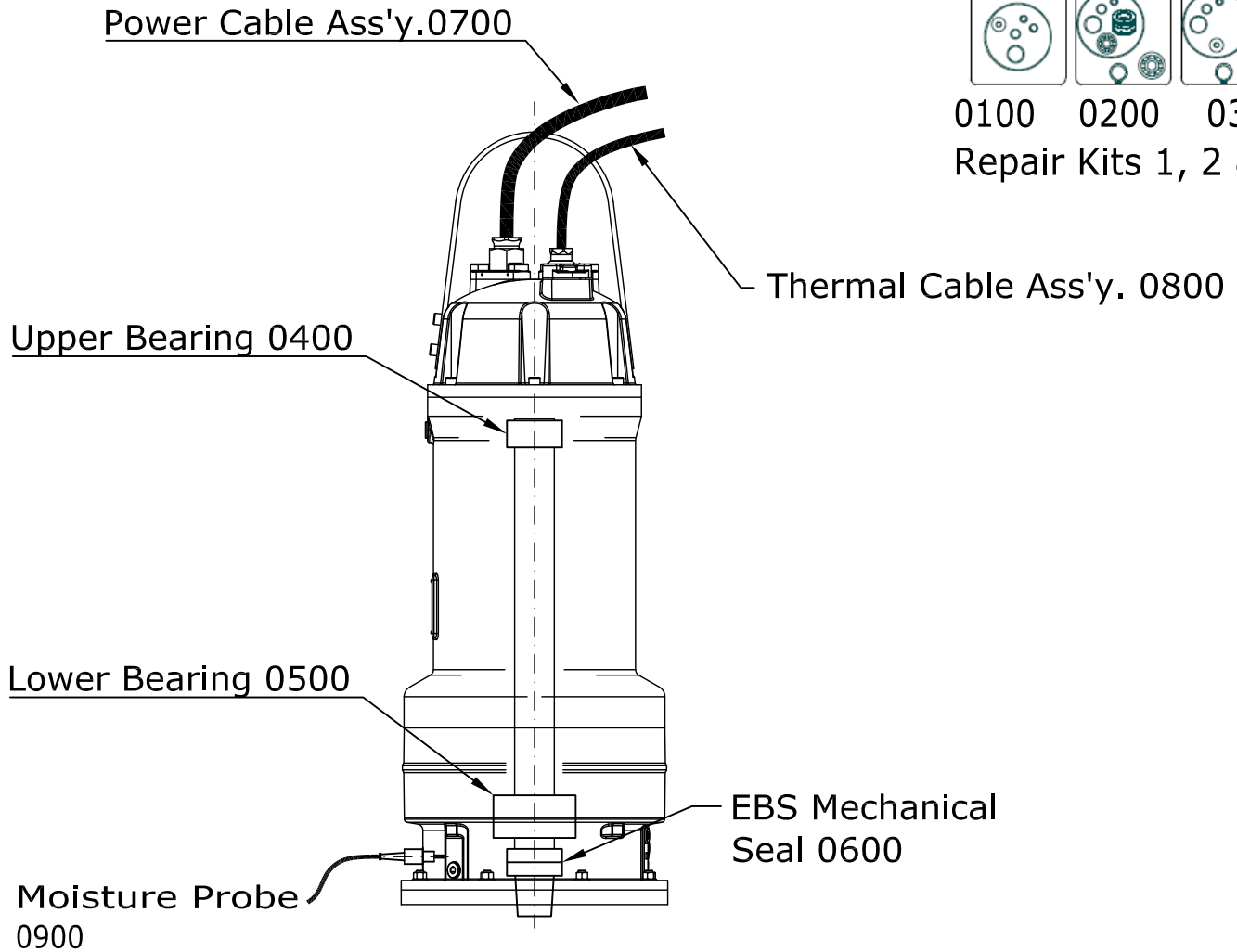
FA10.78Z Pump End
