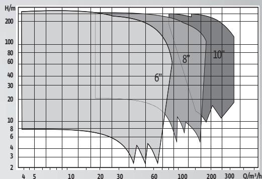
Wilo-SiFire Easy-V
