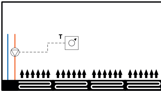
Hall temperature control in an underfloor heating consumer circuit
