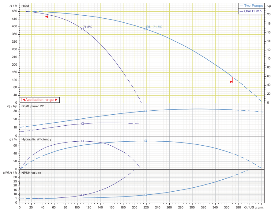
CO-2 Helix 110-06/3
