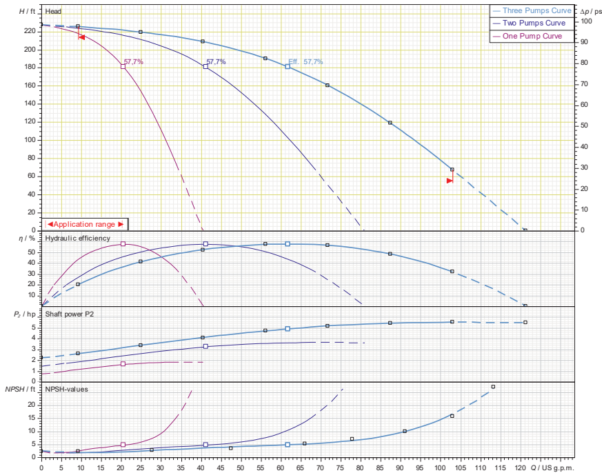
CO-3 HELIX V20-06-1/2/VCE
