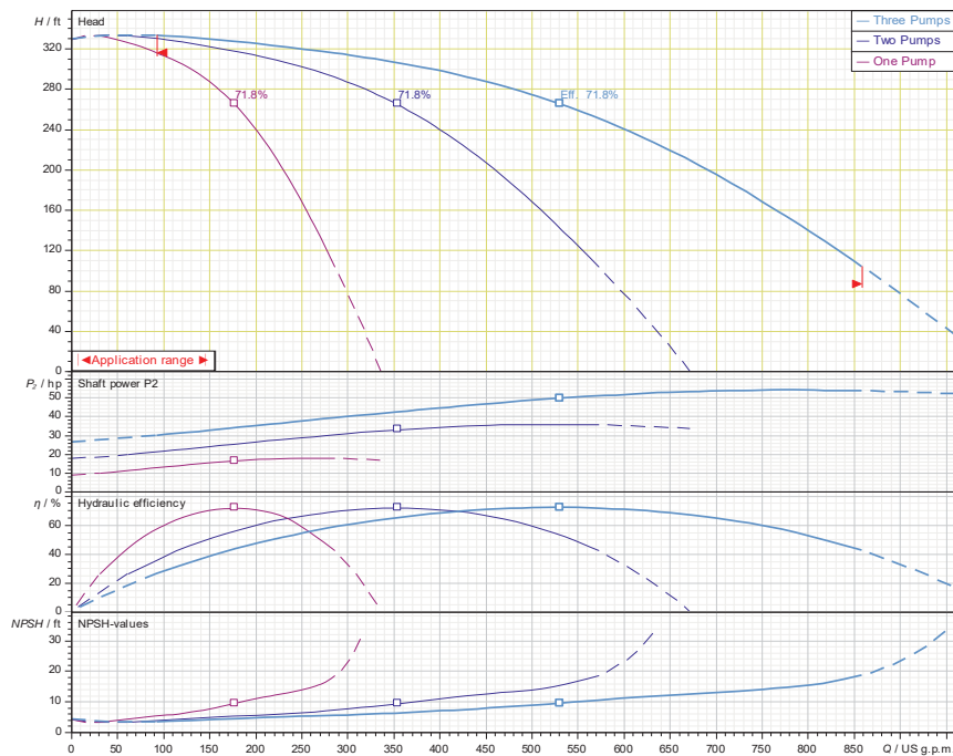
CO-3 Helix 190-03/1
