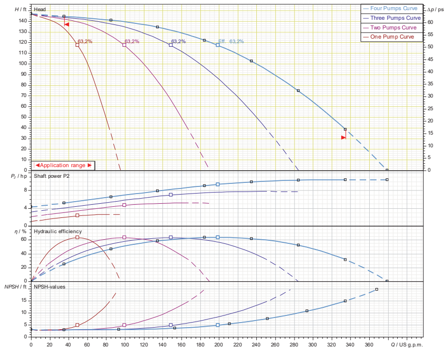
CO-4 HELIX V50-03-1/3/VCE
