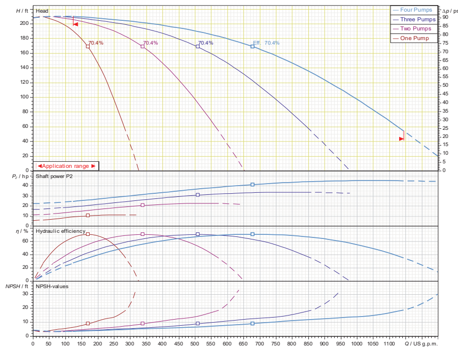
CO-4 Helix 190-02/1
