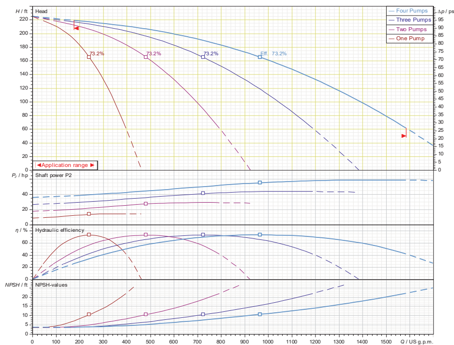
CO-4 Helix 270-02/1
