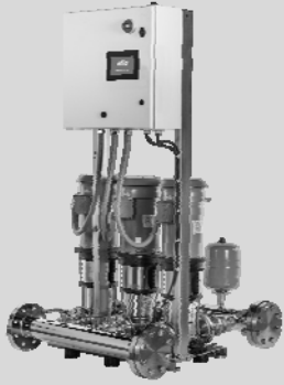
Wilo-CO-Helix Pressure Boosting Systems
