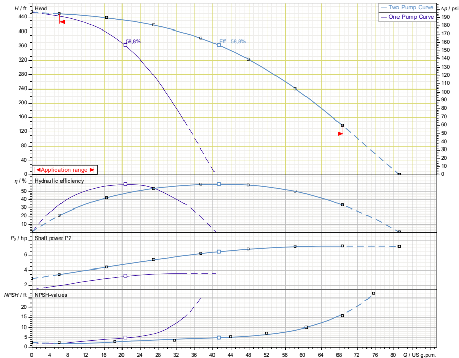
CO-2 HELIX V20-12-1/5/VCE
