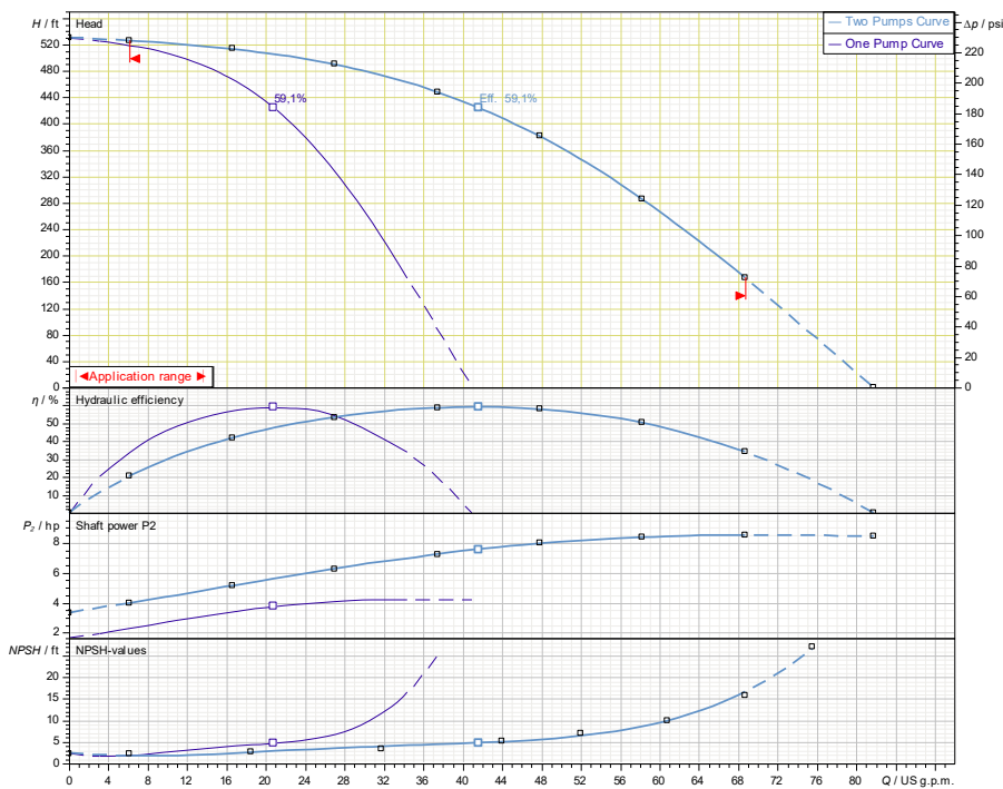
CO-2 HELIX V20-14-1/5/VCE
