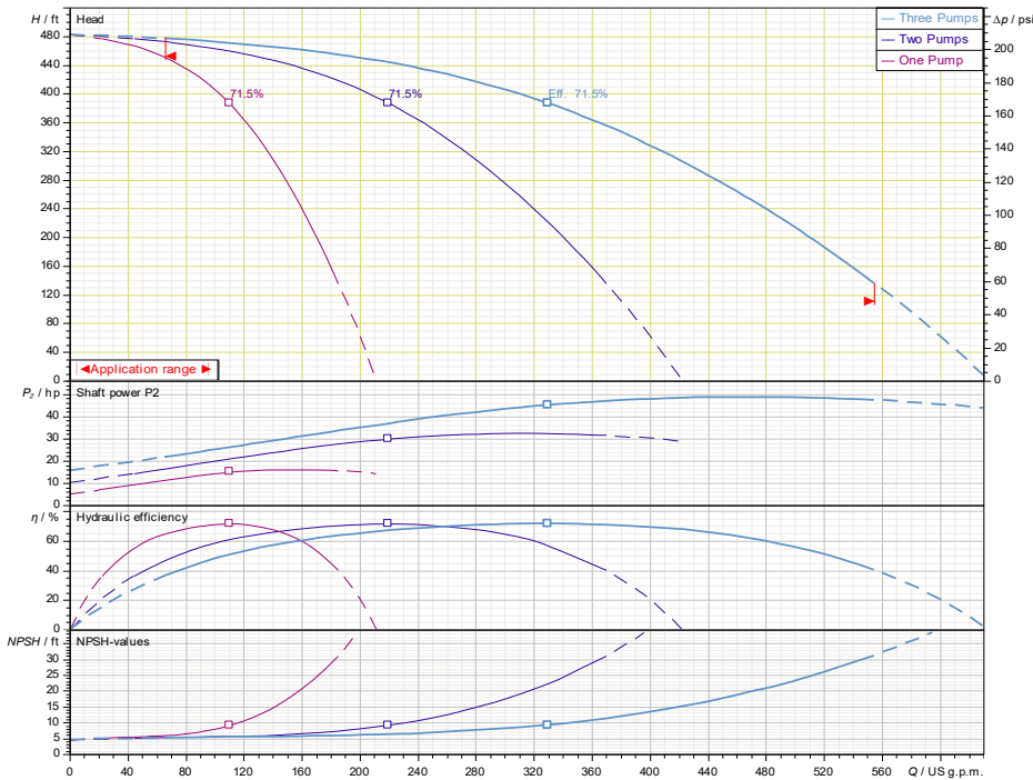
CO-3 Helix 110-06/3
