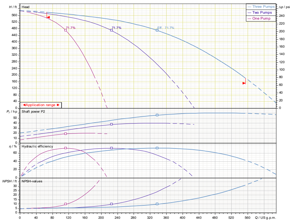
CO-3 Helix 110-07/1
