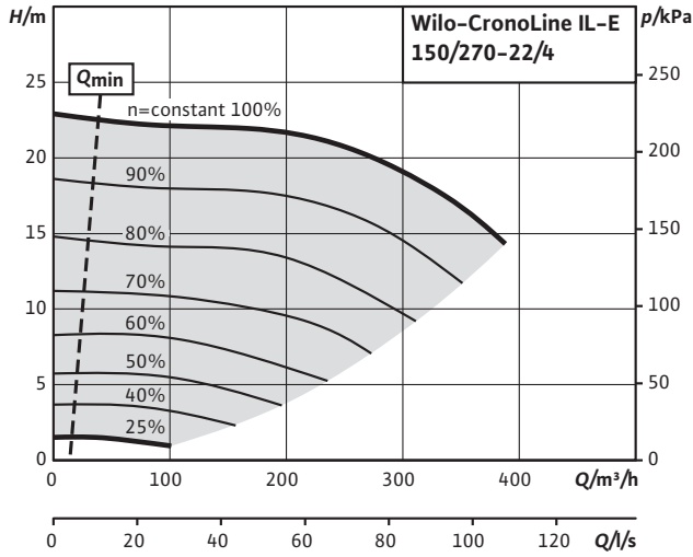
CronoLine-IL-E 150/270-22/4 (4 poli)
