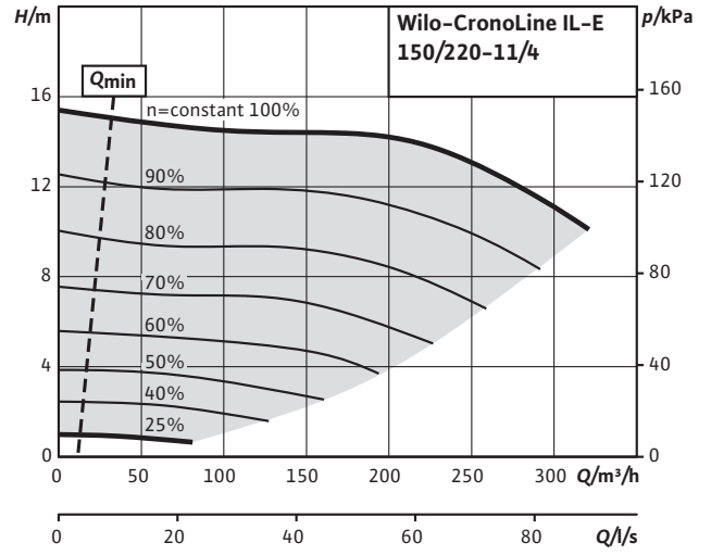
CronoLine-IL-E 150/220-11/4 (4 poli)
