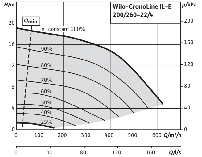
CronoLine-IL-E 200/260-22/4 (4 poli)
